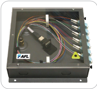
Pre-terminated MTP to LC solution
