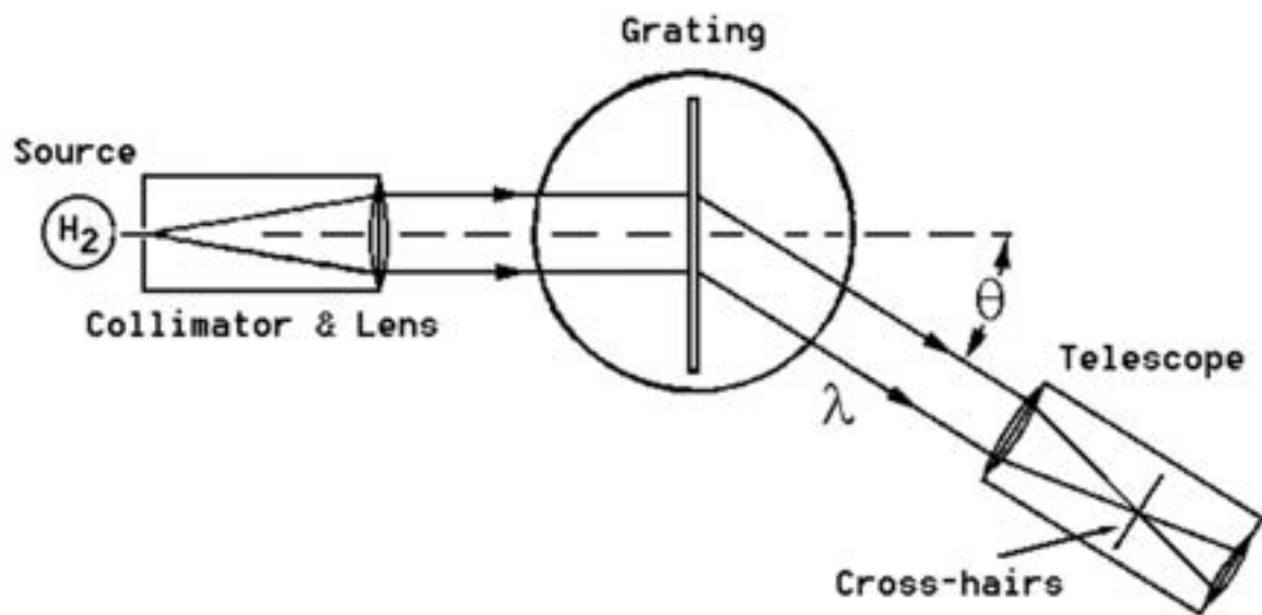
FIGURE 2: SPECTROMETER SETUP
