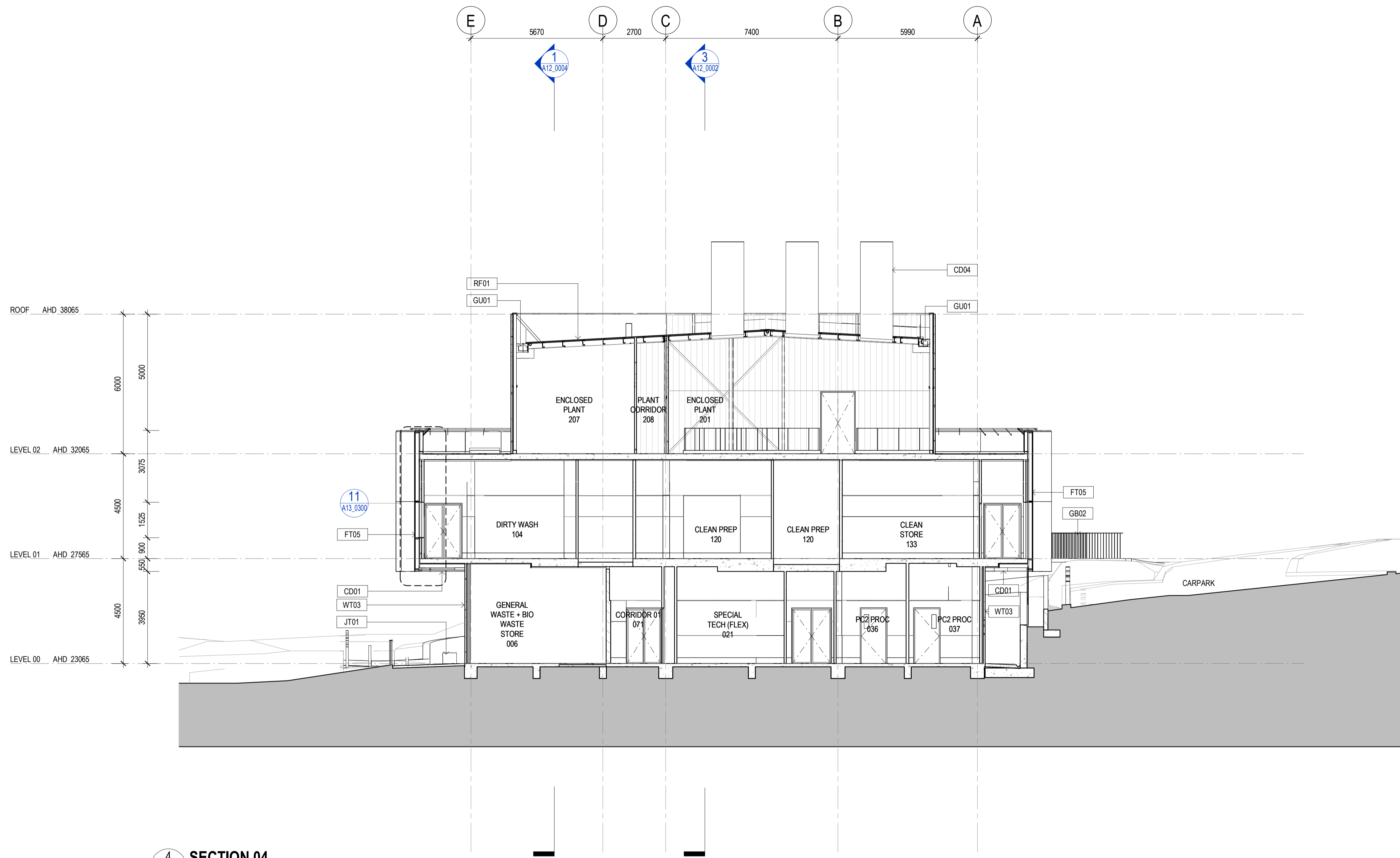
4 SECTION 04 A10_0000 SCALE 1 : 100
