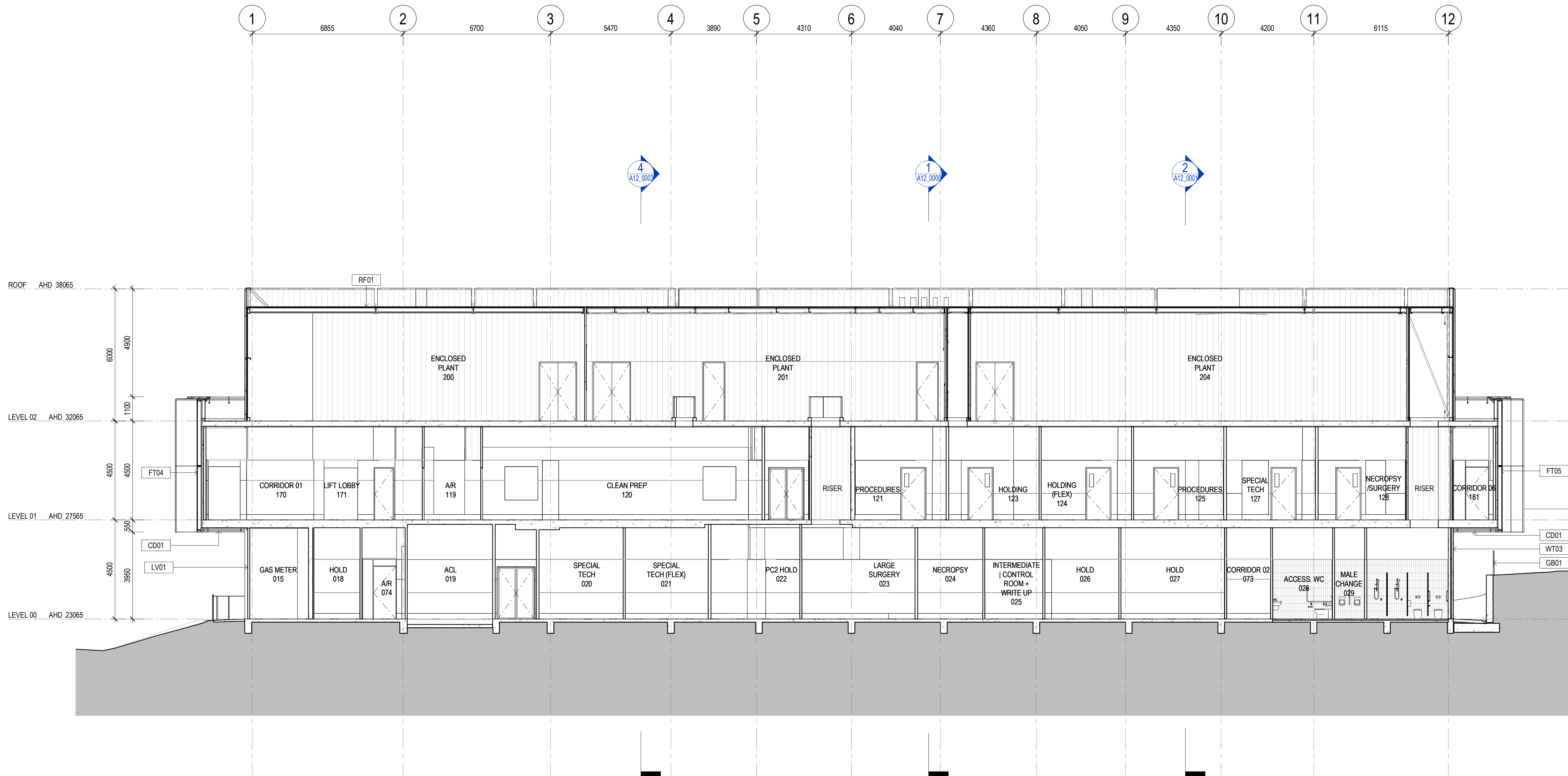
3 SECTION 03 A10_0000 SCALE 1:100
