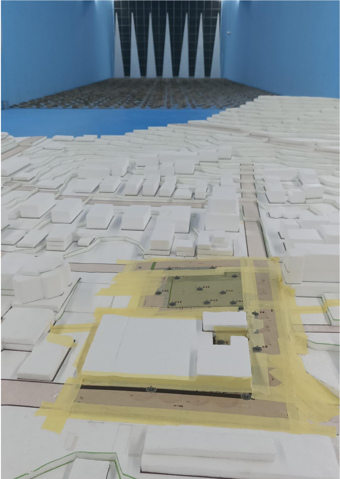
Figure 1f: Photograph of the Wind Tunnel Model (view from the west, existing site conditions)
