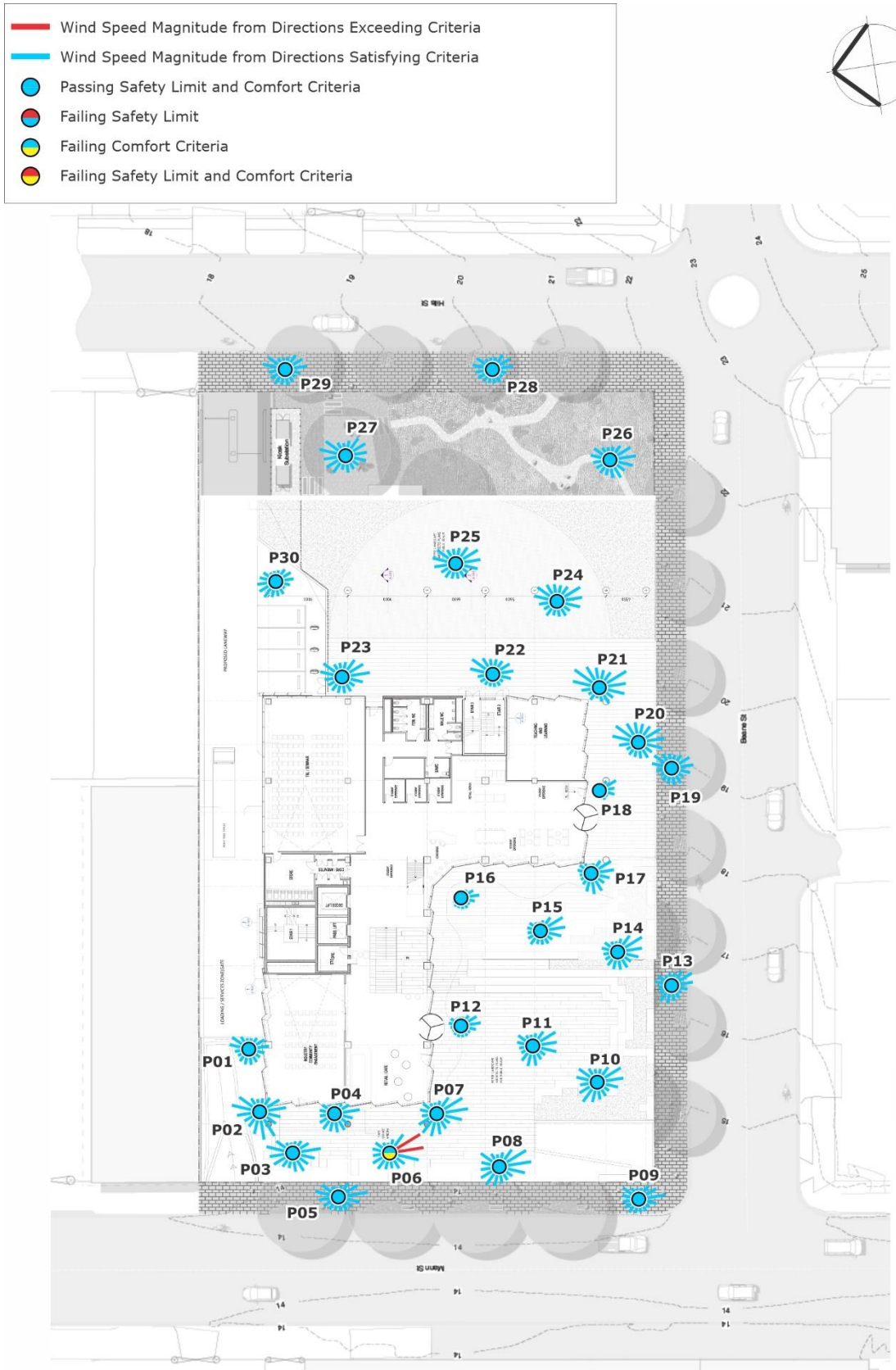
Figure 6: Wind Tunnel Results – Ground Level and Level 1 Plan (results shown without treatments applied)
