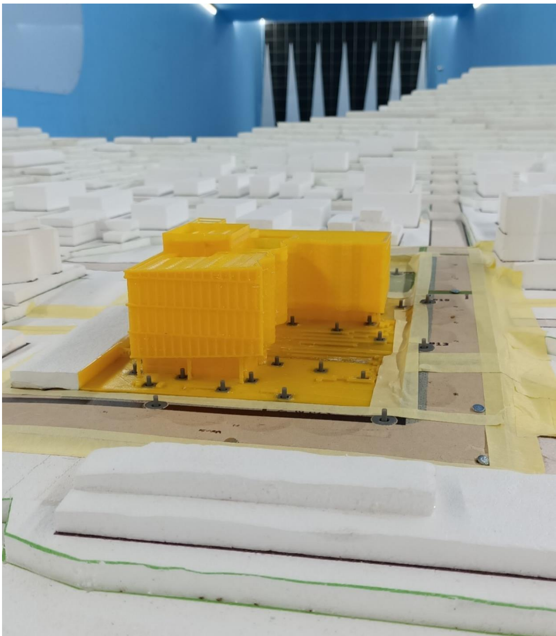
Figure 1a: Photograph of the Wind Tunnel Model (view from the west, proposed site conditions)
