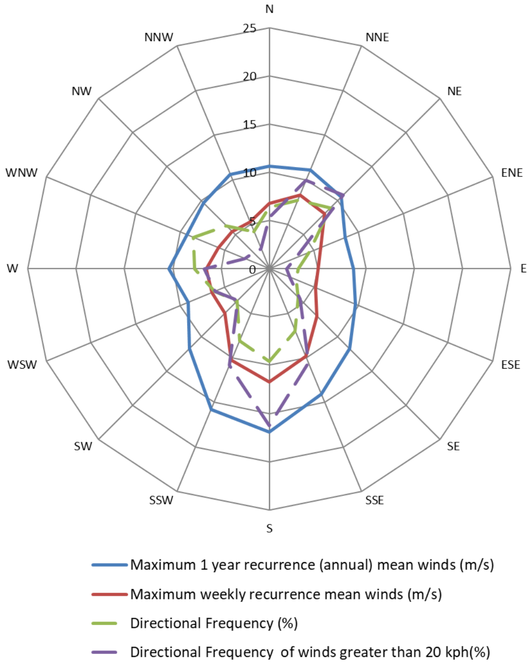
Figure 4: Annual and 5% Exceedance Hourly Mean Wind Speeds, and Frequencies of Occurrence, for the Central Coast Region (at 10m height in standard open terrain)
