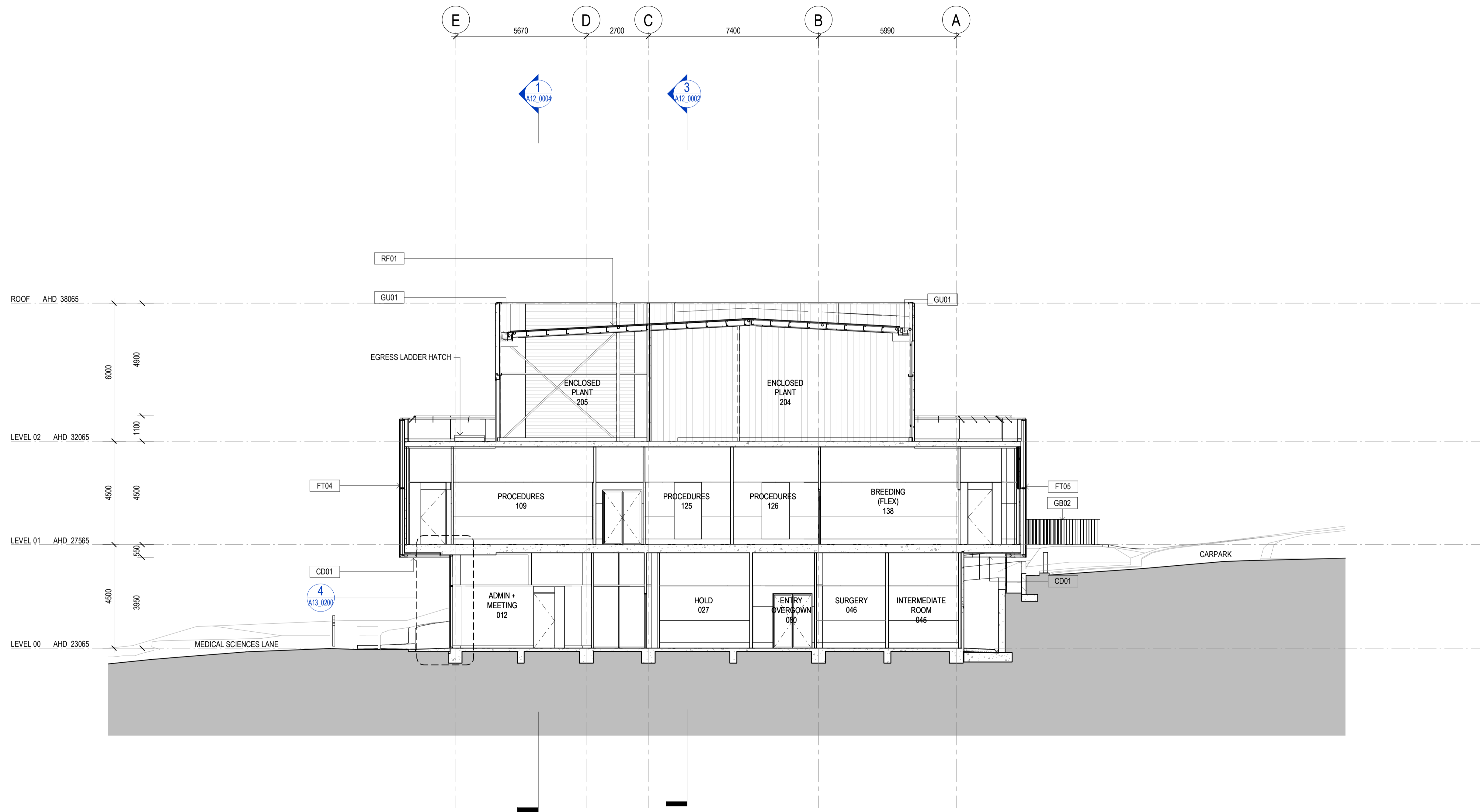
2 SECTION 02 A10_0000 SCALE 1 : 100
